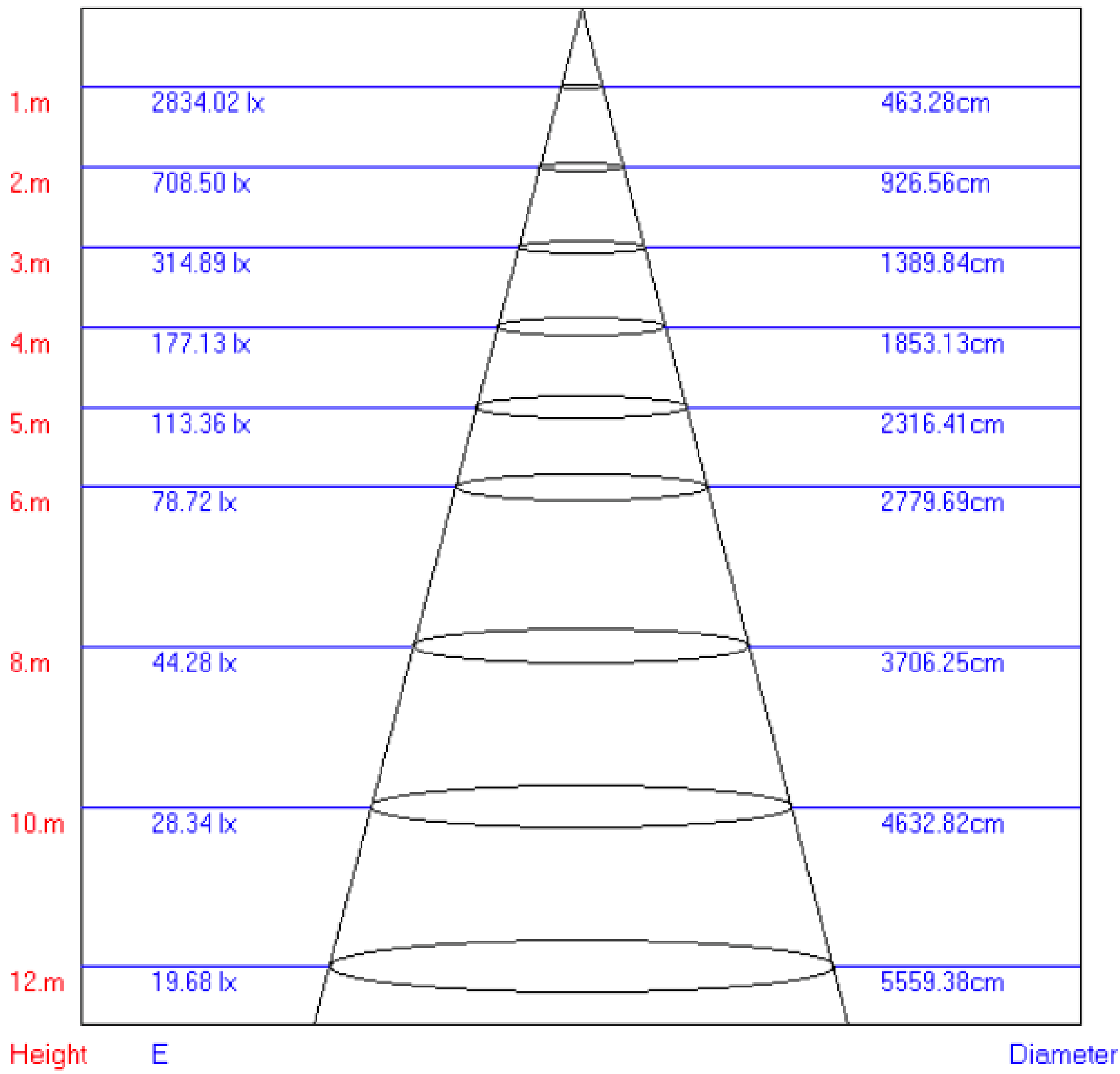
Lux-Distance Curve
